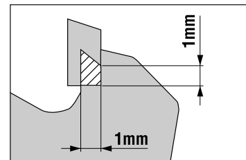
Minimum dimensions of cutting tips of composite circular saw blades in accordance with DIN EN 847-1
